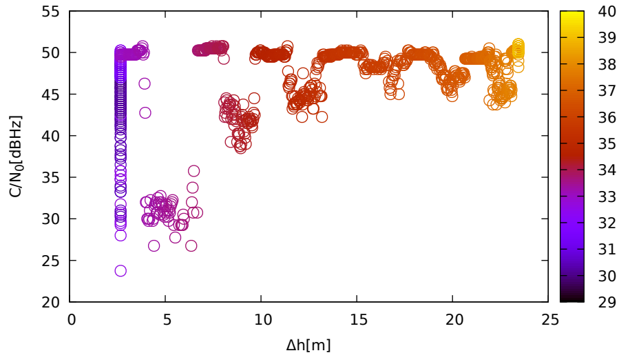
C/N 0 vs height (LeicaGS18 (up) for G31 at L1)
