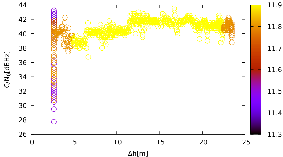
C/N 0 vs height (LeicaGS18 (up) for R02 at L1)
