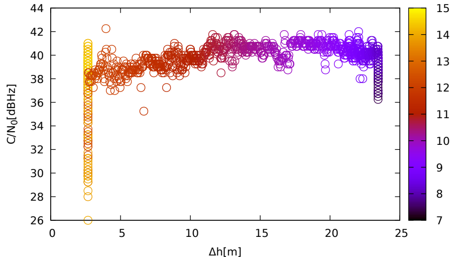
C/N 0 vs height (LeicaGS18 (up) for R03 at L1)
