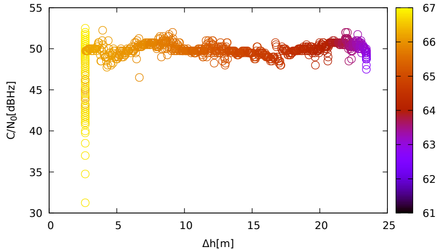
C/N 0 vs height (LeicaGS18 (up) for R09 at L1)
