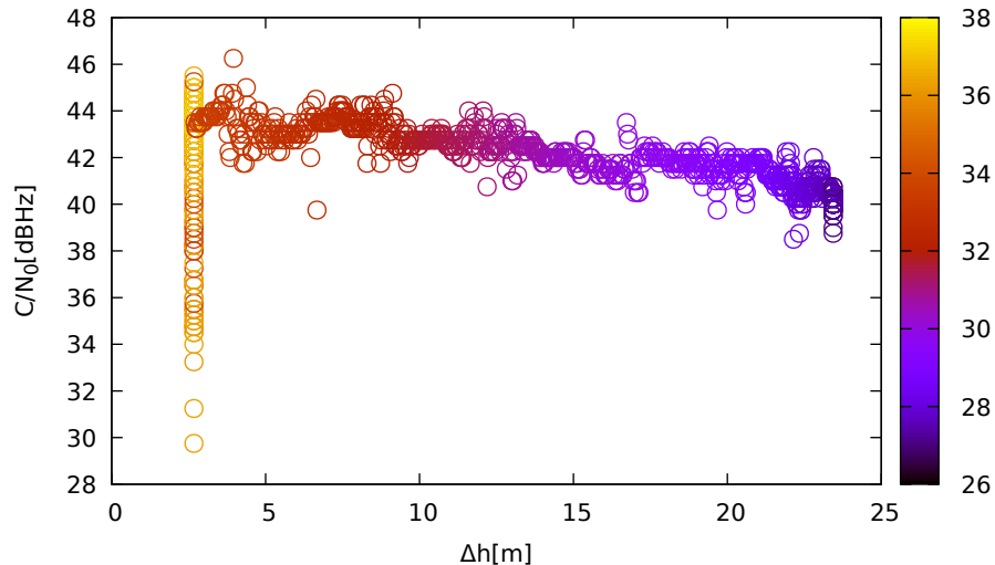
C/N 0 vs height (LeicaGS18 (up) for R10 at L1)
