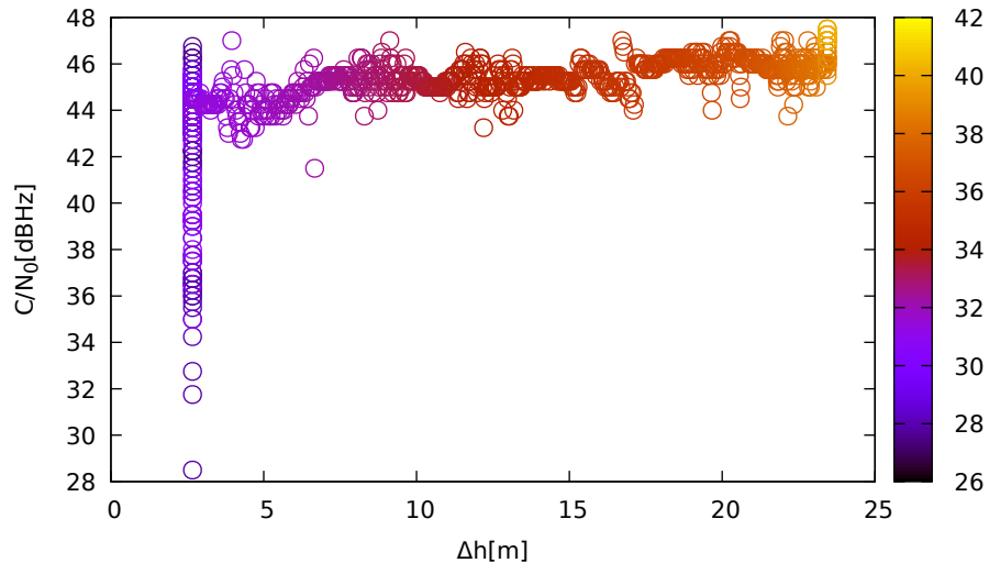
C/N 0 vs height (LeicaGS18 (up) for R16 at L1)
