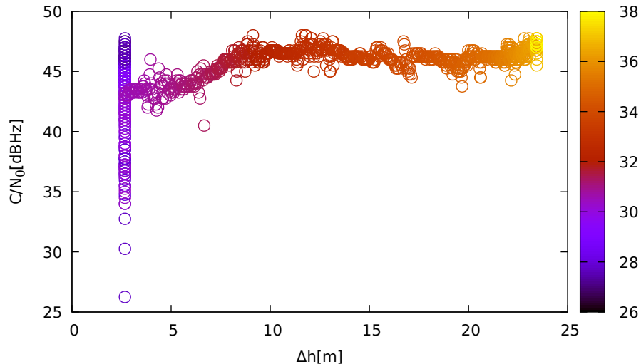
C/N 0 vs height (LeicaGS18 (up) for R18 at L1)
