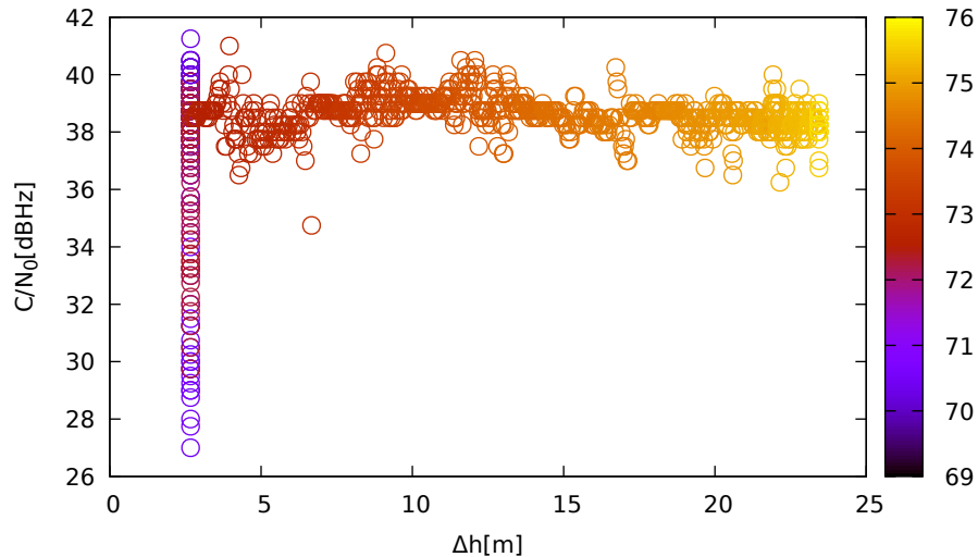
C/N 0 vs height (LeicaGS18 (up) for R19 at L1)
