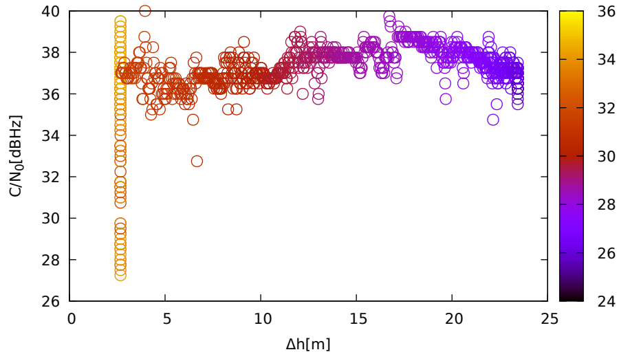
C/N 0 vs height (LeicaGS18 (up) for R20 at L1)
