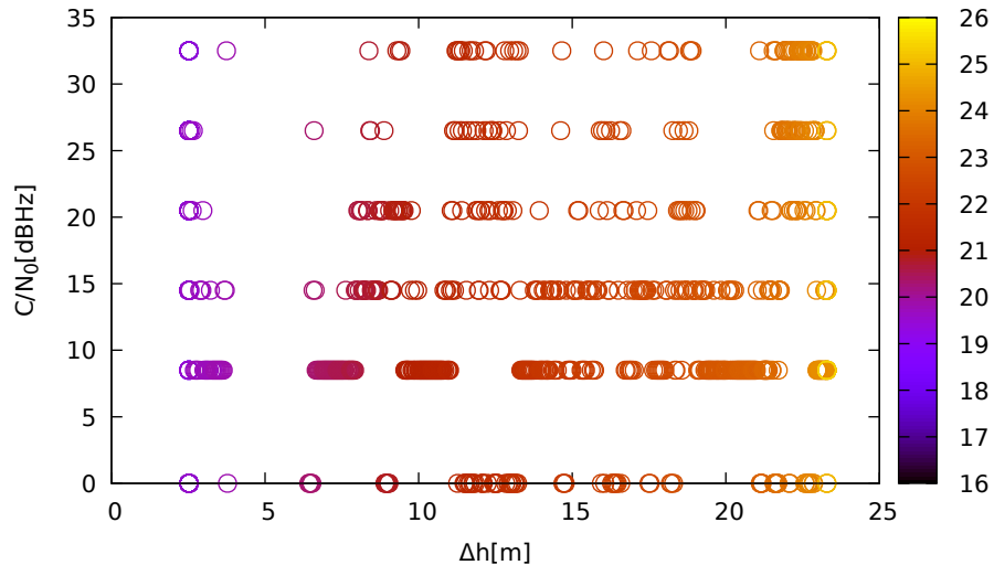
C/N 0 vs height (ublox9 (up) for E01 at L1)
