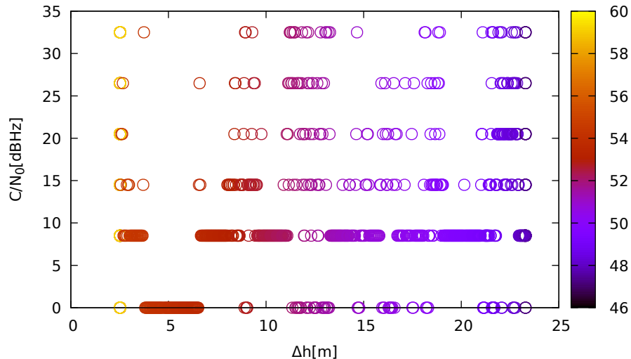
C/N 0 vs height (ublox9 (up) for E18 at L1)
