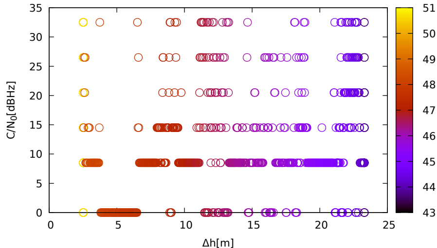
C/N 0 vs height (ublox9 (up) for E24 at L1)
