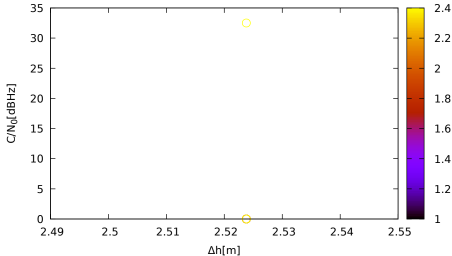
C/N 0 vs height (ublox9 (up) for E25 at L1)
