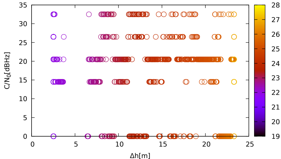
C/N 0 vs height (ublox9 (up) for E26 at L1)
