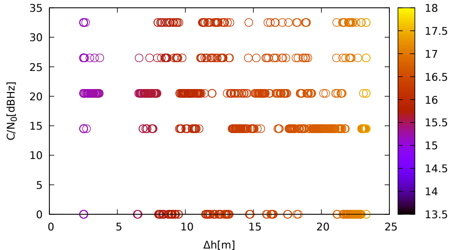
C/N 0 vs height (ublox9 (up) for G05 at L1)
