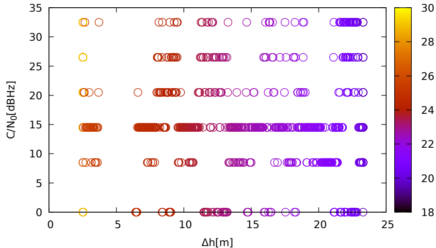
C/N 0 vs height (ublox9 (up) for G16 at L1)
