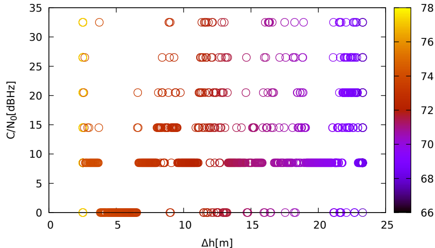
C/N 0 vs height (ublox9 (up) for G18 at L1)
