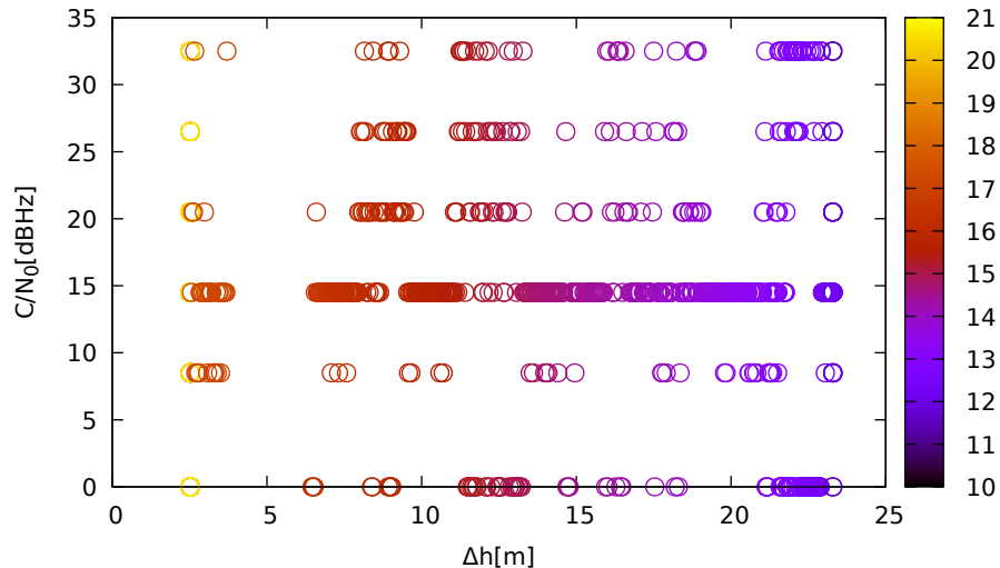
C/N 0 vs height (ublox9 (up) for G20 at L1)
