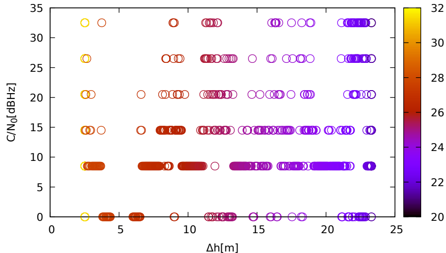
C/N 0 vs height (ublox9 (up) for G21 at L1)
