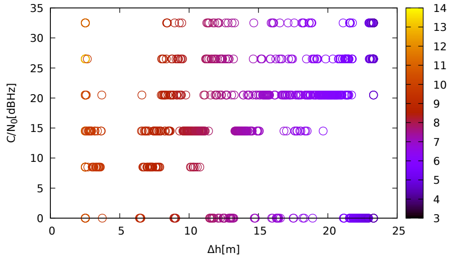
C/N 0 vs height (ublox9 (up) for G23 at L1)
