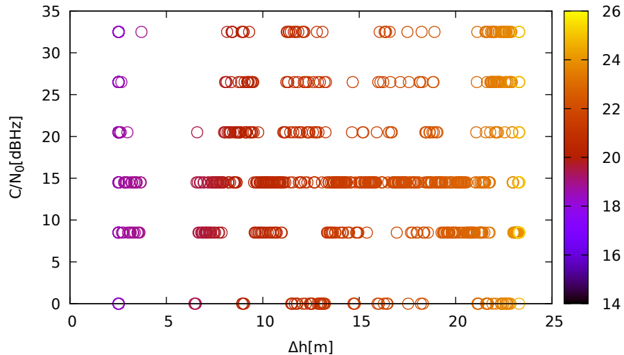
C/N 0 vs height (ublox9 (up) for G25 at L1)
