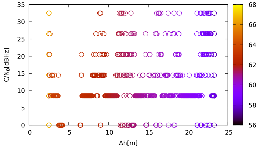
C/N 0 vs height (ublox9 (up) for G26 at L1)
