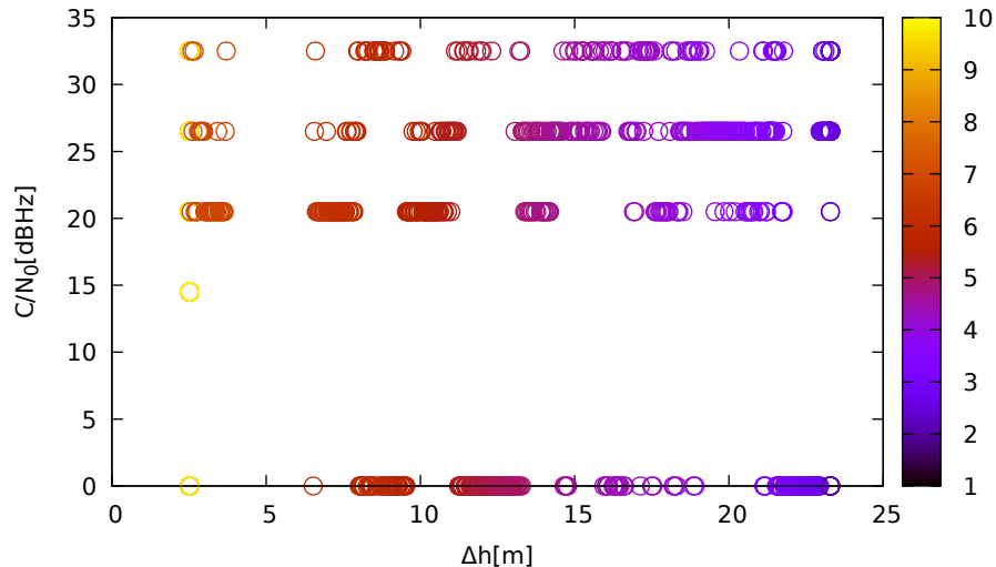
C/N 0 vs height (ublox9 (up) for G27 at L1)
