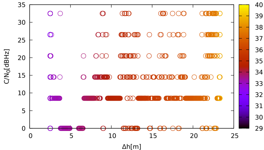
C/N 0 vs height (ublox9 (up) for G31 at L1)
