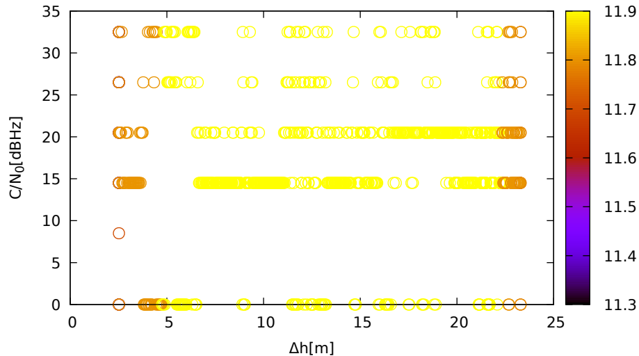
C/N 0 vs height (ublox9 (up) for R02 at L1)
