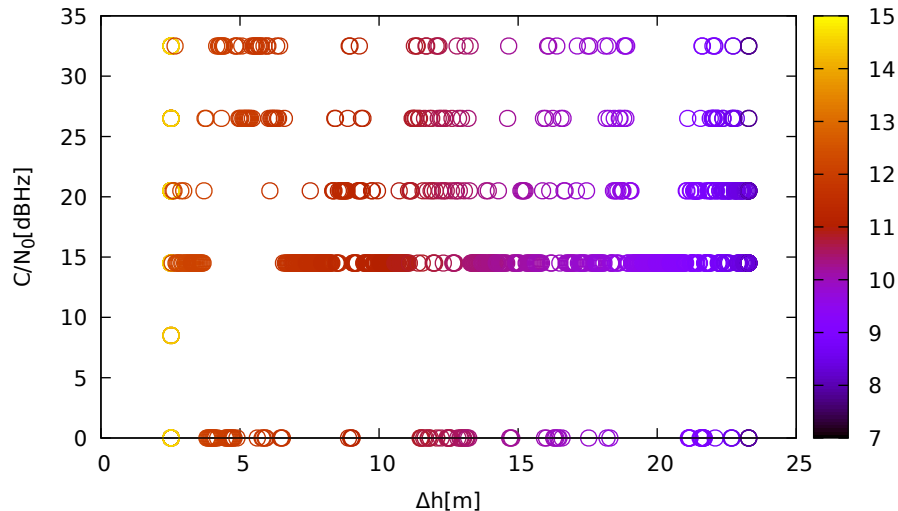
C/N 0 vs height (ublox9 (up) for R03 at L1)
