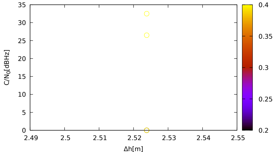
C/N 0 vs height (ublox9 (up) for R04 at L1)
