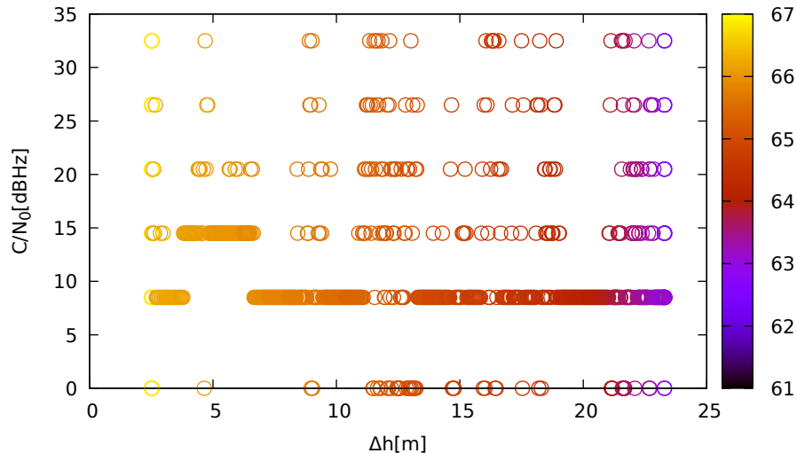
C/N 0 vs height (ublox9 (up) for R09 at L1)
