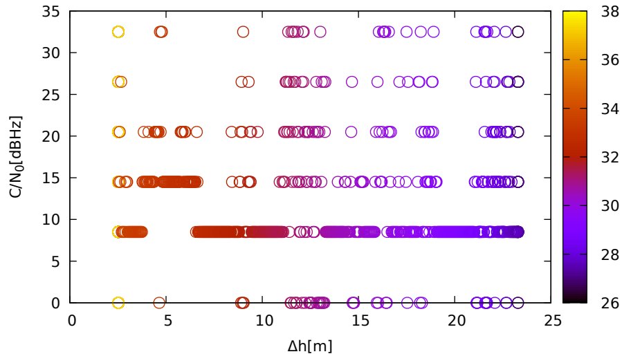
C/N 0 vs height (ublox9 (up) for R10 at L1)
