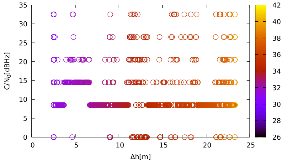
C/N 0 vs height (ublox9 (up) for R16 at L1)
