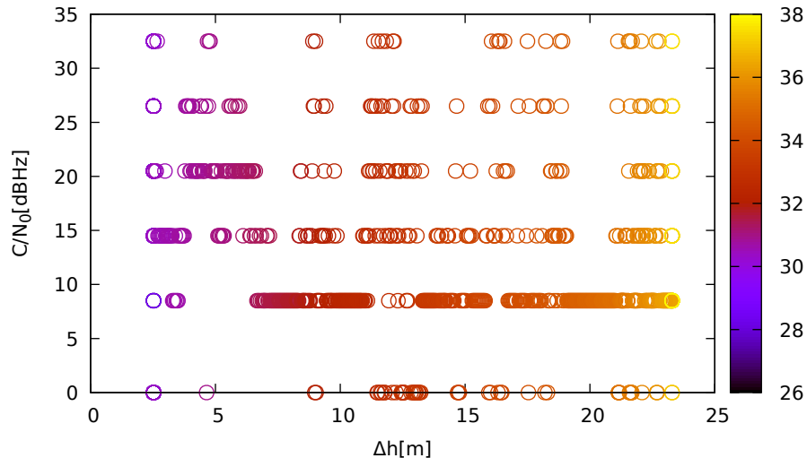
C/N 0 vs height (ublox9 (up) for R18 at L1)
