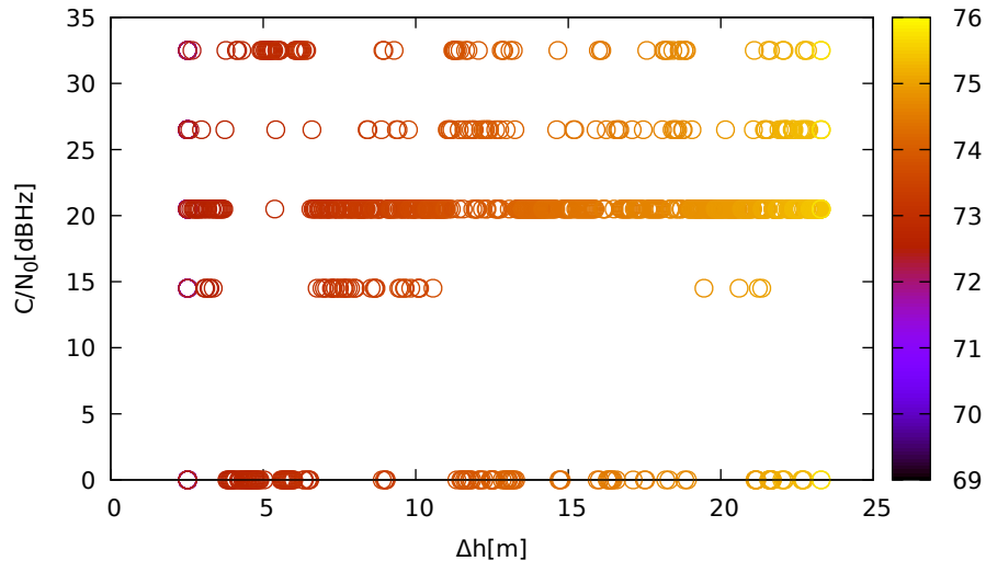
C/N 0 vs height (ublox9 (up) for R19 at L1)
