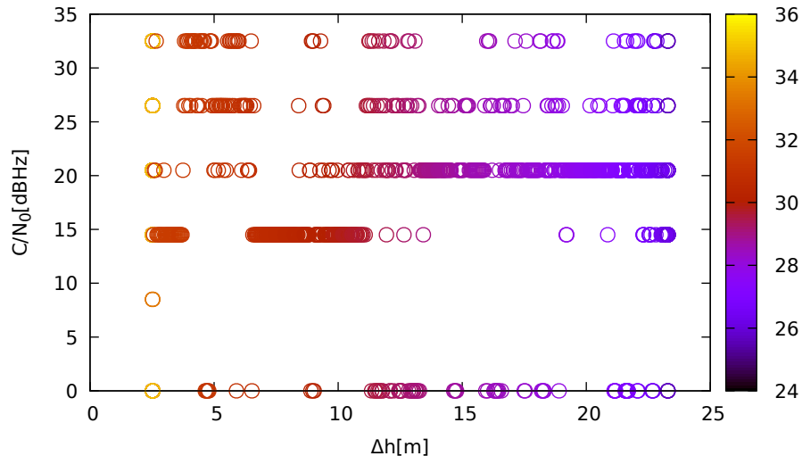
C/N 0 vs height (ublox9 (up) for R20 at L1)
