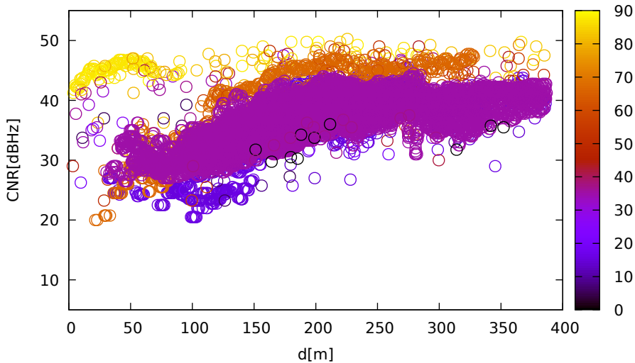
CNR vs distance (Javad for 123 at L1)
