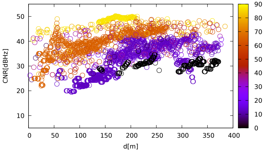
CNR vs distance (Javad for 125 at L1)
