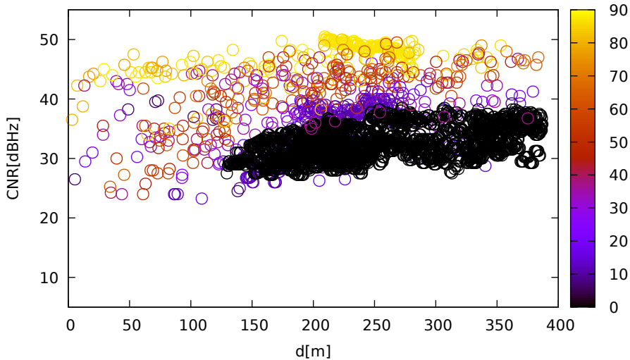
CNR vs distance (Javad for 126 at L1)
