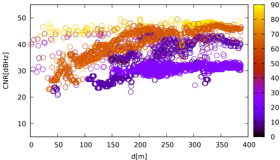
CNR vs distance (Javad for 127 at L1)
