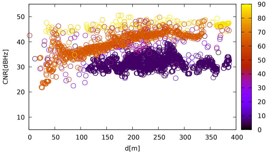
CNR vs distance (Javad for 128 at L1)
