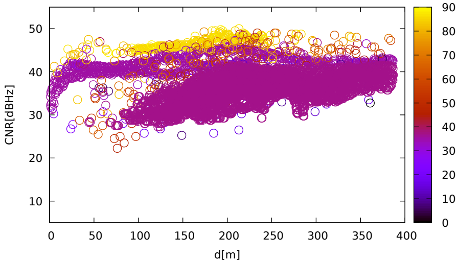
CNR vs distance (Javad for 136 at L1)
