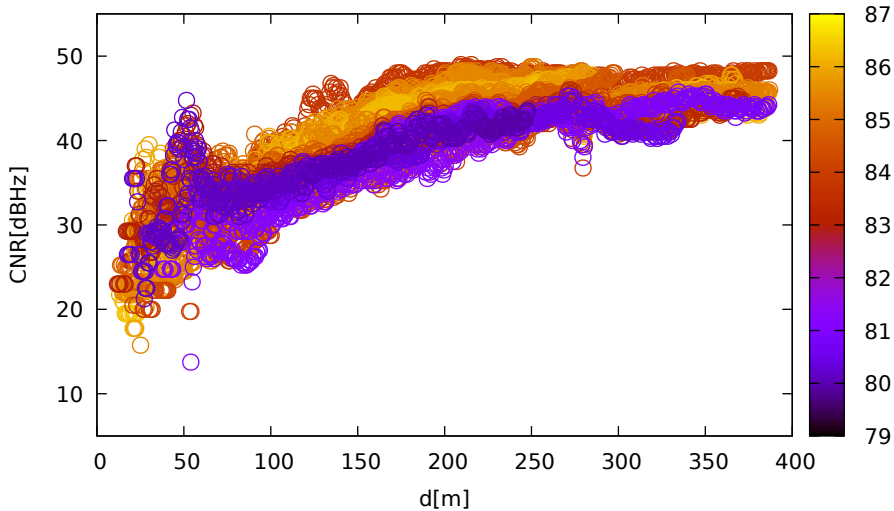
CNR vs distance (Javad for C27 at L1)
