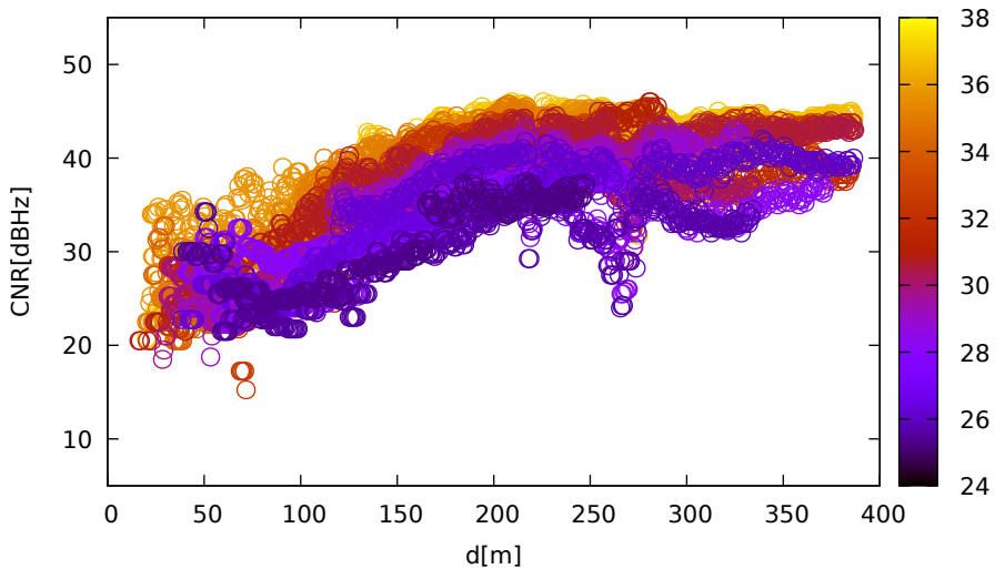
CNR vs distance (Javad for C28 at L1)
