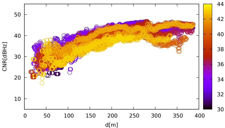
CNR vs distance (Javad for C30 at L1)
