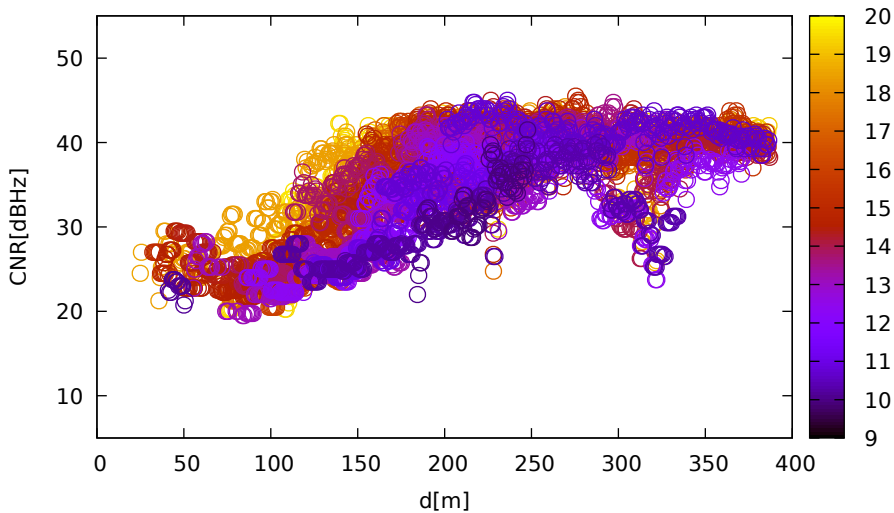
CNR vs distance (Javad for E01 at L1)
