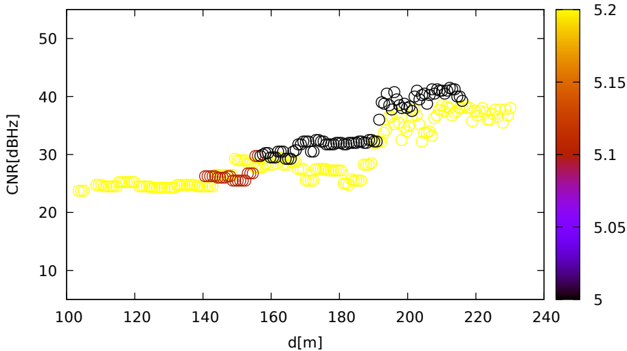
CNR vs distance (Javad for E05 at L1)
