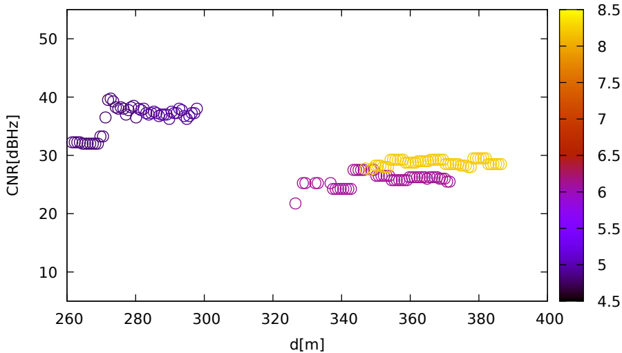
CNR vs distance (Javad for E11 at L1)
