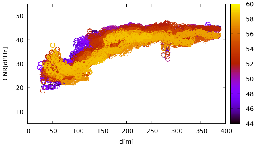
CNR vs distance (Javad for E12 at L1)
