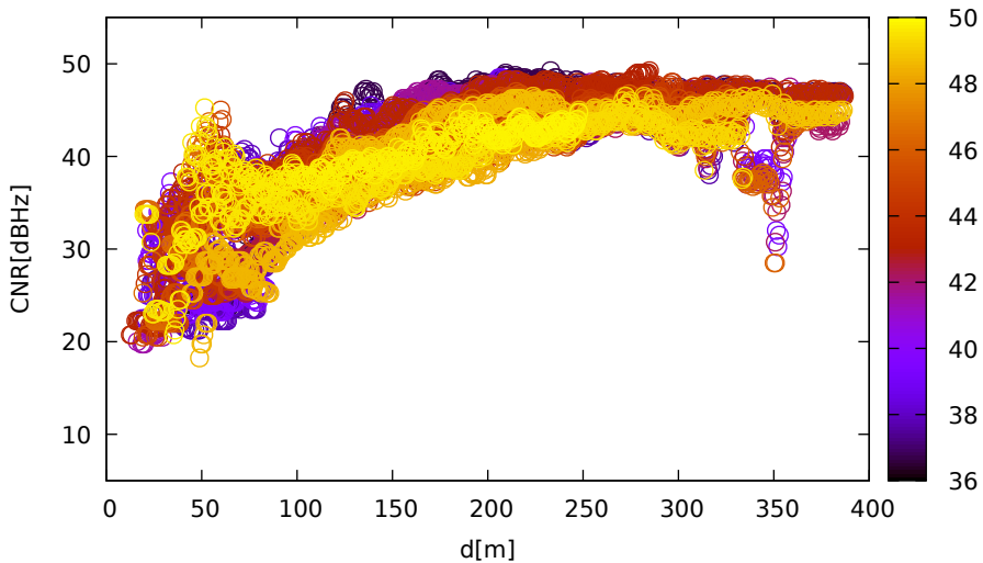
CNR vs distance (Javad for E14 at L1)
