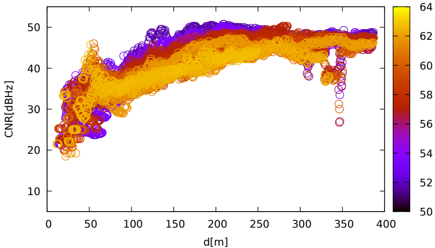
CNR vs distance (Javad for E24 at L1)
