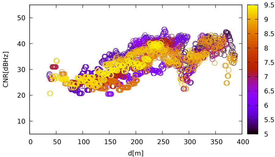
CNR vs distance (Javad for E25 at L1)
