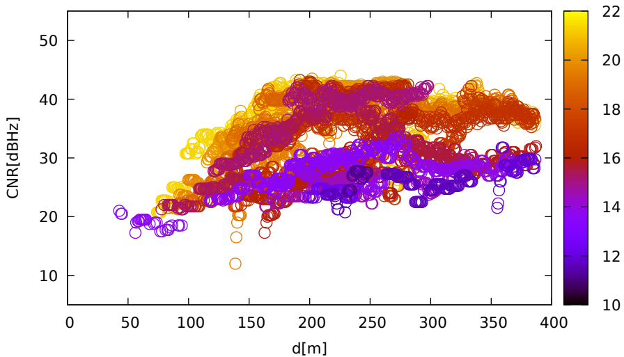
CNR vs distance (Javad for E26 at L1)
